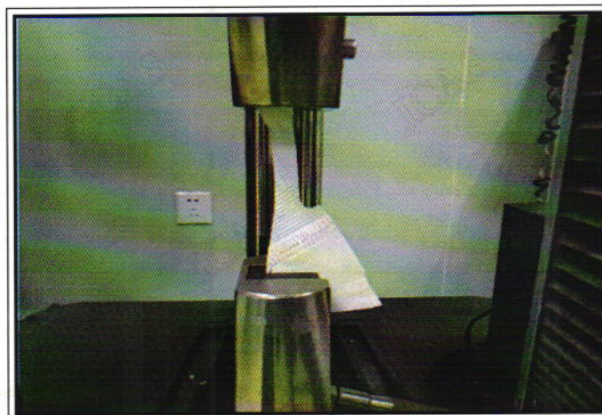
试验中 During the test
